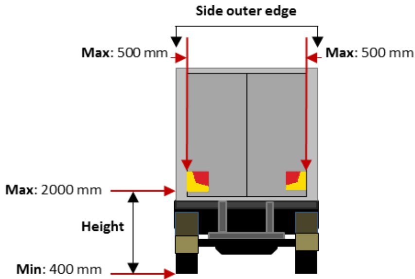
Figure 1. Positioning dimensions
